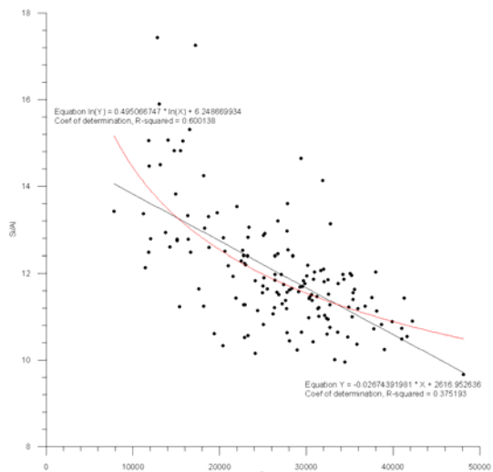
Figure 3.31. XRF based data showing the relationship between the Si signal and the Si/Al ratio.
