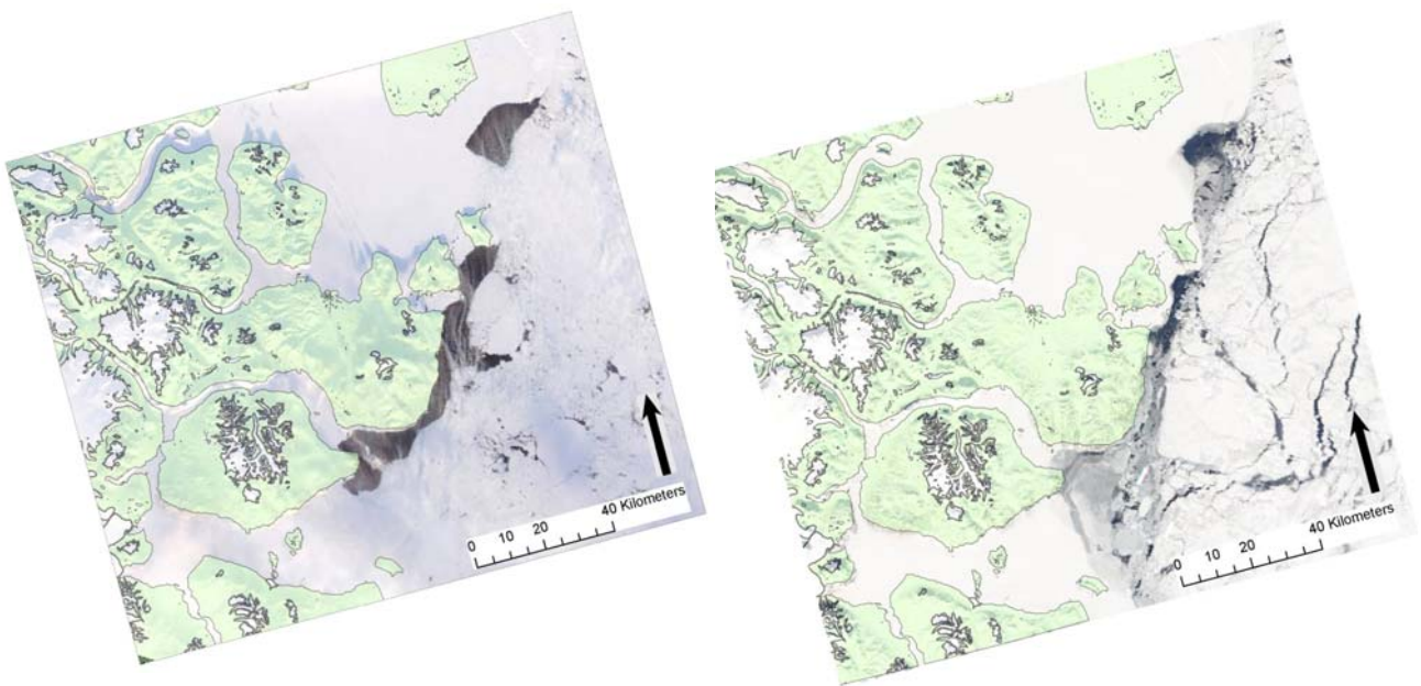
Figure 2.9. Modis satellite images of the expedition area, showing the ice coverage on 29 February 2008 (left panel) and 29 April 2008 (right panel).
