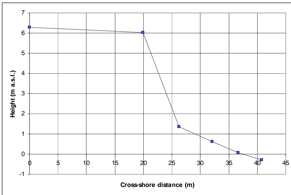
Figure A1.6 Cross-shore beach profile C1 (28-08-2008; Day-of-year 241)
