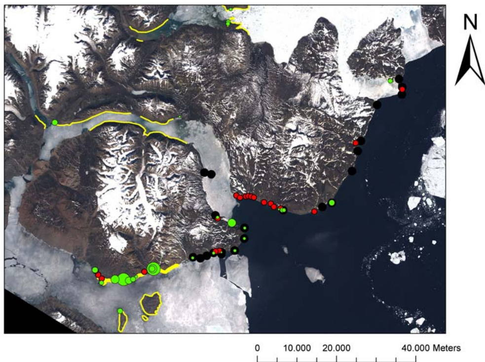
Figure 3.10. Geomorphologic map with distribution of Thule Culture winter houses. Legend: winter house (green dot), beach ridge system (red dot), pocket beach fringing gneiss formations (yellow line), and basalt capes (black dots).
