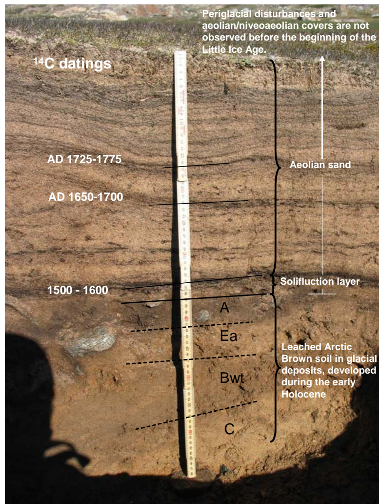
Figure 3.28. Soil profile at Eskimovig, showing an Early Holocene soil, influenced by periglacial activity during the Little Ice Age.
