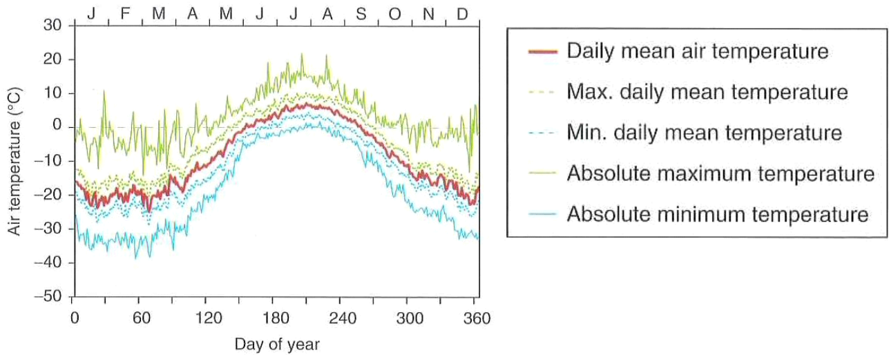
Figure 2.3 Daily mean temperatures and absolute maximum and minimum temperatures at Zackenberg over the period 1996-2005 (Hansen et al., 2008).
