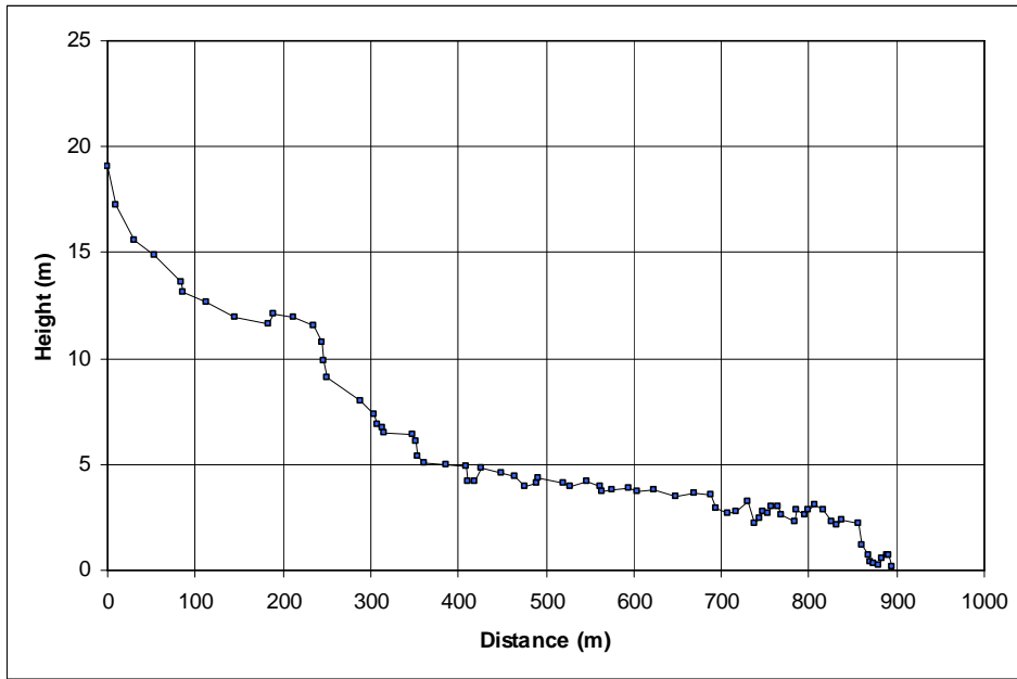
Figure A1.5 Cross-delta profile (28-08-2008; Day-of-year 241)
