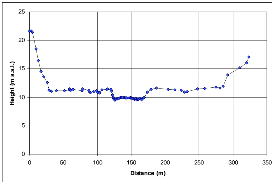
Figure A2.3 Southern river profile (01-09-2008; Day-of-year 245)
