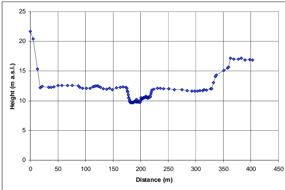
Figure A2.2 Central river profile (01-09-2008; Day-of-year 245)
