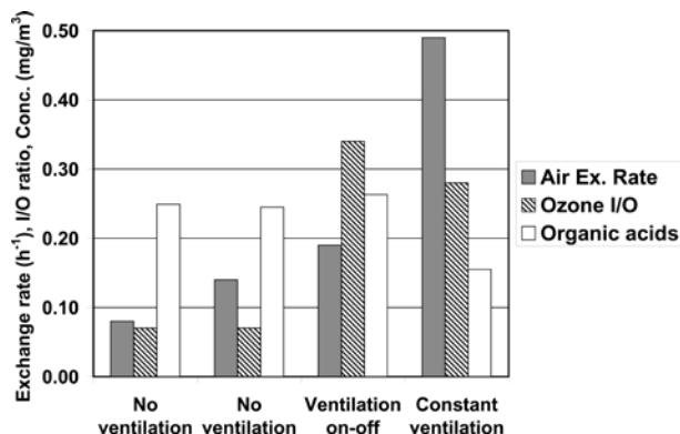
Figure 3. The air exchange ( \text{h}^{-1} ), ozone indoor/outdoor ratio, and organic acids concentration ( \text{mg}/\text{m}^3 ) for four different monitoring periods at the Arnamagnæan Institute's archive with four different ventilation rates.
