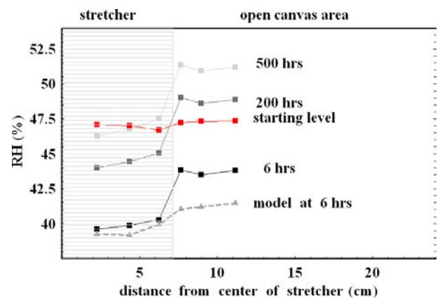
Figure 10. Relative humidity profile measured along the canvas in the third experiment (with buffering by absorbent wood and wall) after 0, 6, 200 and 500 hours from the setting up of the thermal gradient, and the calculated profile after 6 hours.
