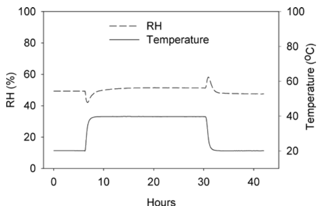
Figure 9. Temperature and relative humidity conditions within a microclimate package containing an oak panel and Artsorb.
