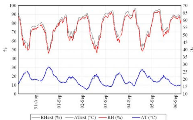
Figure 6. The internal and external relative humidity (RH) and ambient temperature (AT) are almost identical during the open summer of 2005, indicating minimal buffering
