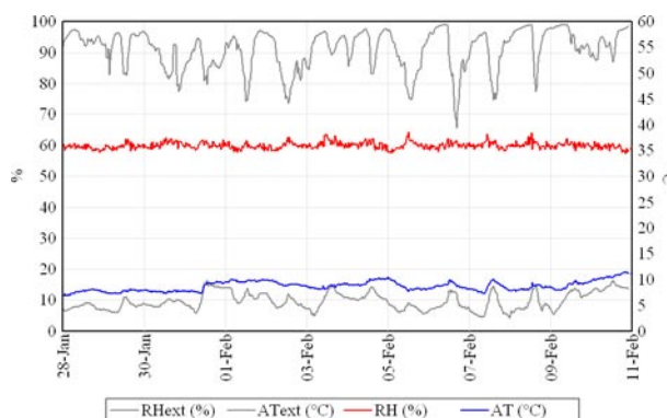
Figure 9. Internal and external relative humidity (RH) and ambient temperature (AT) in the winter of 2005 during enclosure and dehumidification, demonstrating the high level of buffering
