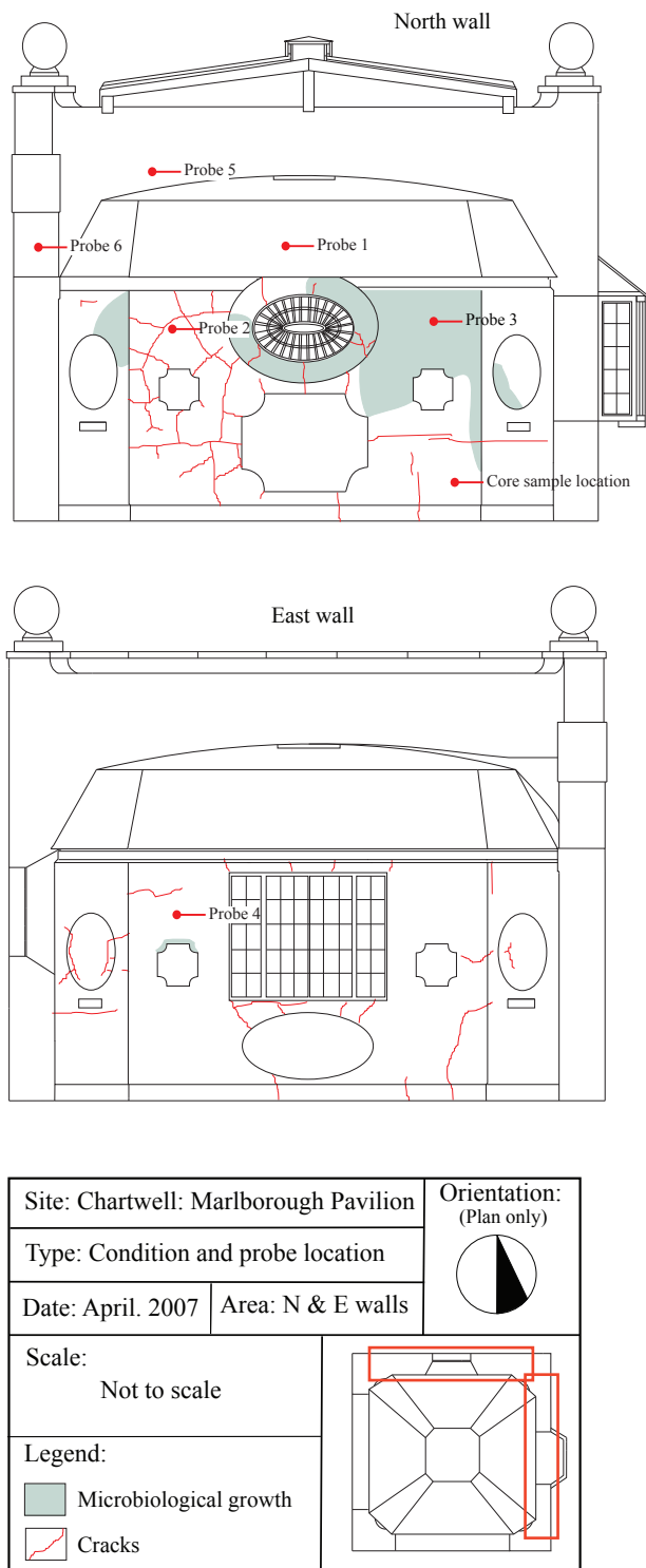
Figure 4. Plan and elevations with the patterns of damage and the location of the monitoring probes and core sample
