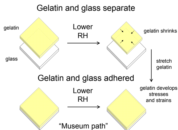
Figure 1. Extreme environmental changes cause damage due to the differential expansion and contraction of materials. If the RH around a free gelatin layer is lowered, it shrinks and no strains or stresses are generated. If it is adhered to a glass plate that does not respond to RH changes, however, it cannot shrink because the glass is stiffer, stronger, and thicker. Stresses and strains develop in the gelatin even though there is minimal dimensional change. The glass plate develops little strain (its size is minimally different from a free glass plate) but develops stresses equal and opposite to those in the gelatin layer. This example demonstrates why the stress-strain behaviour and dimensional response to RH change of the individual materials must be known to predict the behaviour of an object, and why dimensional measurements alone cannot be used to determine the state of an object or to predict behaviour.
