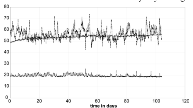
Figure 3. Graph showing the relative humidity and temperature inside and outside a framed, glazed and back-boarded oil painting on stretched canvas kept in an unconditioned gallery at Tate Britain (Tate) at a temperature around 20°C (lowest line on graph). The stability of RH inside a frame (the continuous line) is well documented.
