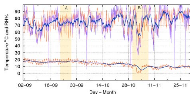
Figure 18. The simulated indoor RH is considerably stabilised by the RH buffer applied to the walls. Now, the inside RH variation never exceeds that outdoors.
