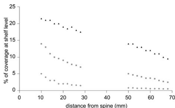
Figure 7. Dust deposition onto the top edges of books with different gap sizes between the top of book and the shelf above. Glass slides were placed along top edges of books and analysed after 30 days exposure. Dust deposition is expressed as a percentage of that occurring on the shelf at the front of the book to account for different positions of books within a library. Two different behaviours are observed, with larger gap sizes showing almost linear decay, whilst smaller gap sizes show more exponential decay.
