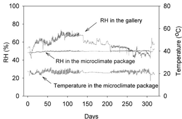
Figure 12. Environmental conditions inside and outside a microclimate package for an Italian renaissance panel painting (with Artsorb) while on loan to two museums.
