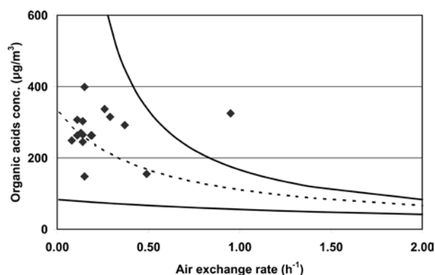
Figure 2. The concentration of organic acids (μg/m 3 ) at different air exchange rates, modelled for a 120 m 3 room. The internal emission of organic acids – emission from furniture, building materials, or the collection itself - is assumed constant at 20 mg/h. The relation is modelled for three different environments: a highly reactive room with the acid surface removal rate of 2 h -1 (low curve), a normal room with the acid surface removal rate of 0.5 h -1 (dotted curve), and a room with no surface removal at all (upper curve). For the latter model ventilation is the only removal mechanism. The single data points represent measurements from real museum stores similar to the model room.
