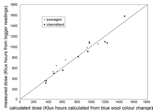
Figure 2. Accuracy of Blue Wool Dosimeter measurements in real situations. The dose calculated from blue wool colour change is plotted against dose determined by illumination measurement for both the intermittent and the more accurate averaged measurements.
