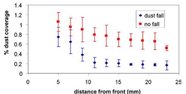
Figure 7. Fig Traditional dust falls reduce the penetration of dust, and rates of dust deposition, in book shelves in the Great Library at Audley End House (English Heritage). The deposition rate is measured as % coverage over a thirty day period.
