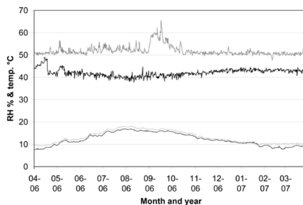
Figure 2. Halls C and B showing the two different climatic zones in the stores (hall C 50% RH (grey trace) and hall B 40% RH (black trace)). Hall C represents the other two halls A and D, since they are being dehumidified by the same plant.
