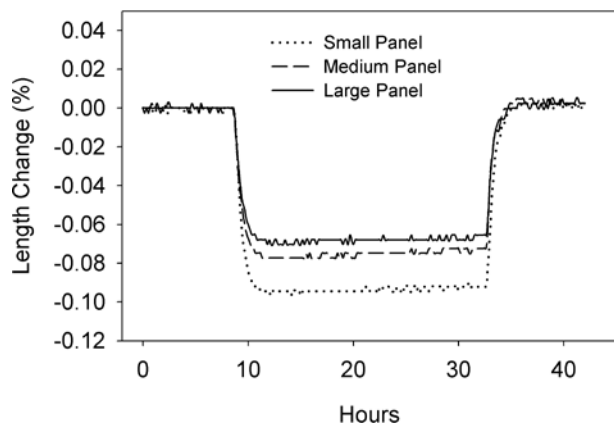
Figure 11. Percent change in length ( \Delta L/L \times 100 ) of oak panels inside microclimate packages (with Rhapid Gel) during 20^\circ\text{C} variations.
