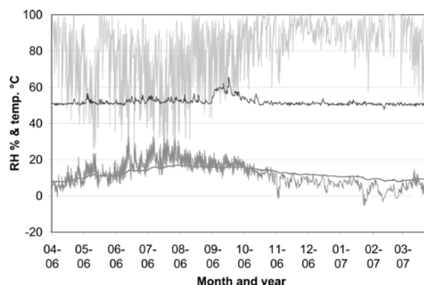
Figure 3. RH and temperature (black trace) in hall C and outdoors (grey trace) during 2006.
