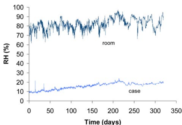
Figure 1. Conditions inside standard 'EH1' showcase at Pevensey Castle. The RH is maintained close to 20% for eleven months.
