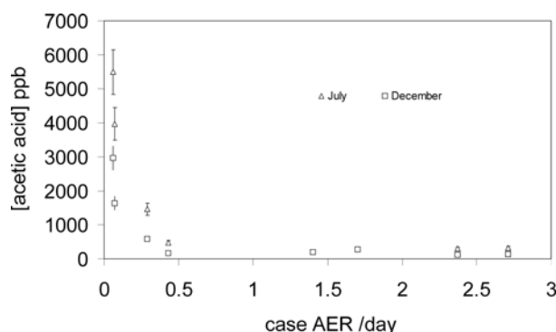
Figure 8. Ethanoic acid concentrations in a series of cases at the British Museum. Concentrations increase sharply when AER drops below 0.5 per day. Summer concentrations are higher, because higher temperature and RH increase the emission rate from medium density fibreboard.
